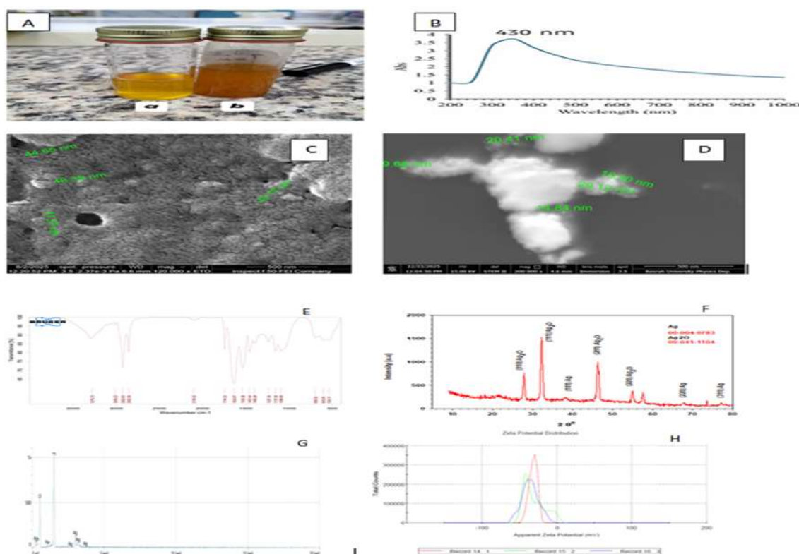
Figure 2. Characterization of Sinapis alba -derived AgNPs: (A) color change during synthesis; (B) UV-Vis absorption spectrum; (C) SEM and (D) TEM images; (E) FTIR spectrum; (F) XRD pattern; (G) EDX analysis; and (H) zeta potential. (Prepared by Authors, 2026).
