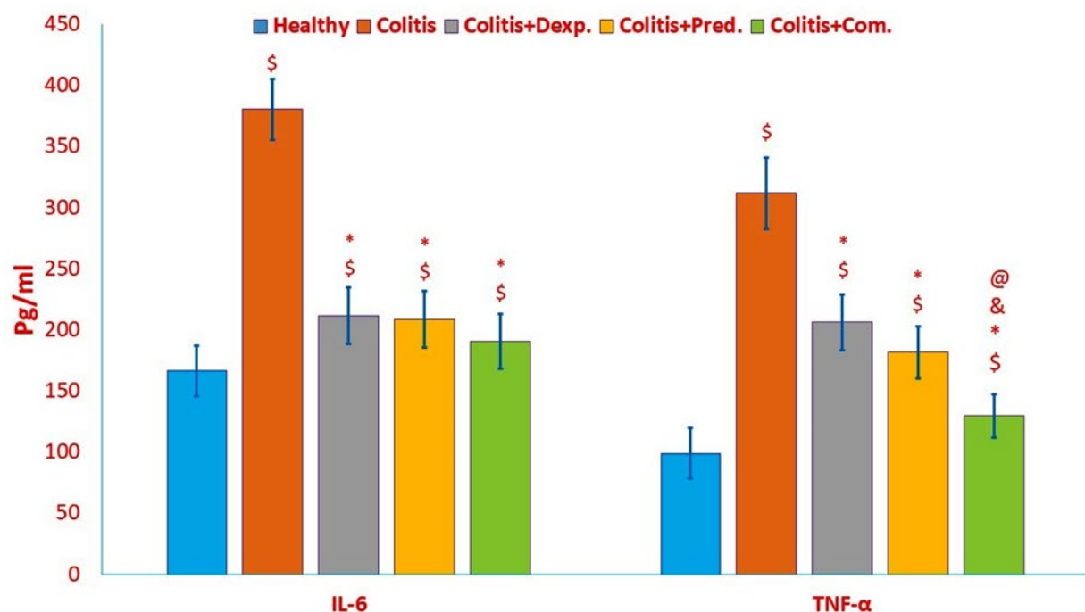
Figure 4. The effect of therapeutic approaches on the levels of pro-inflammatory cytokines in the colonic homogenate of experimental rats. The findings are shown as mean \pm SD ($ P <0.05 versus healthy rats; * P <0.05 versus PBS-treated IBD rats; & P <0.05 versus dexpanthenol-treated RA rats; @ P <0.05 versus prednisolone-treated rats).
